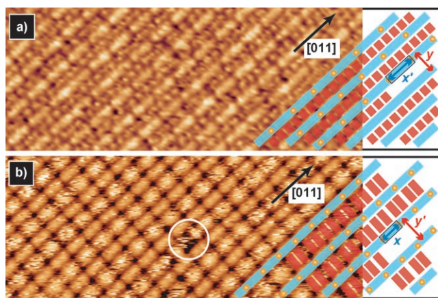
Figure 3. STM topographs ( 250 \text{ Å} \times 100 \text{ Å} ) of the hierarchical assembly of a) P2/C1 and b) P1/C2 (with missing C2 defect circled). These mixtures demonstrate the possibility of tuning the geometric parameters x and y (see Figure 1 b) independently by modular replacement of the molecular building blocks.
